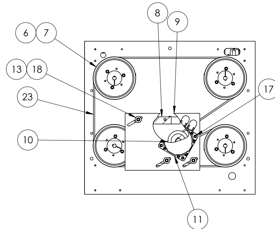
BOTTOM VIEW DRIVE SYSTEM
